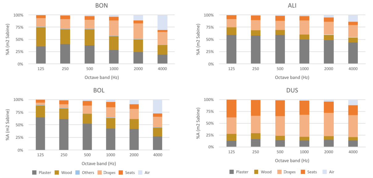
Fig. 3 – Percentage of equivalent absorption area of each layer in unoccupied conditions
