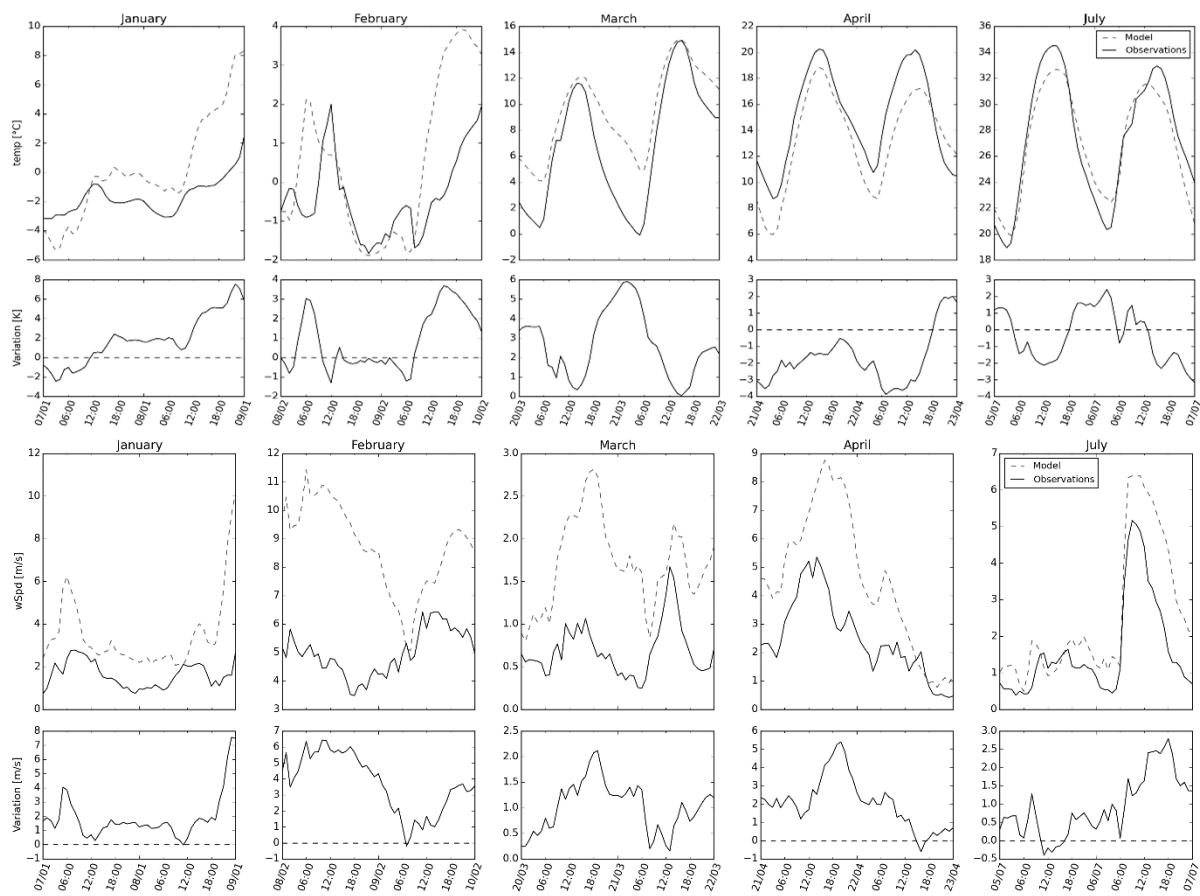
Fig. 6a, 6b – Model vs. Observations for 2 m Temperature (top) and Wind Speed (bottom)
